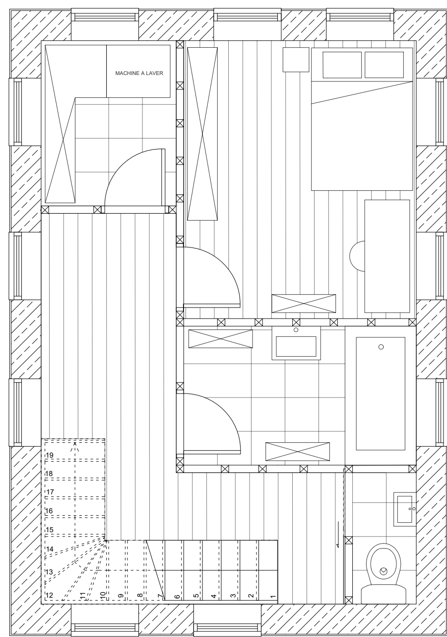
PLAN R+1 1 / 50
