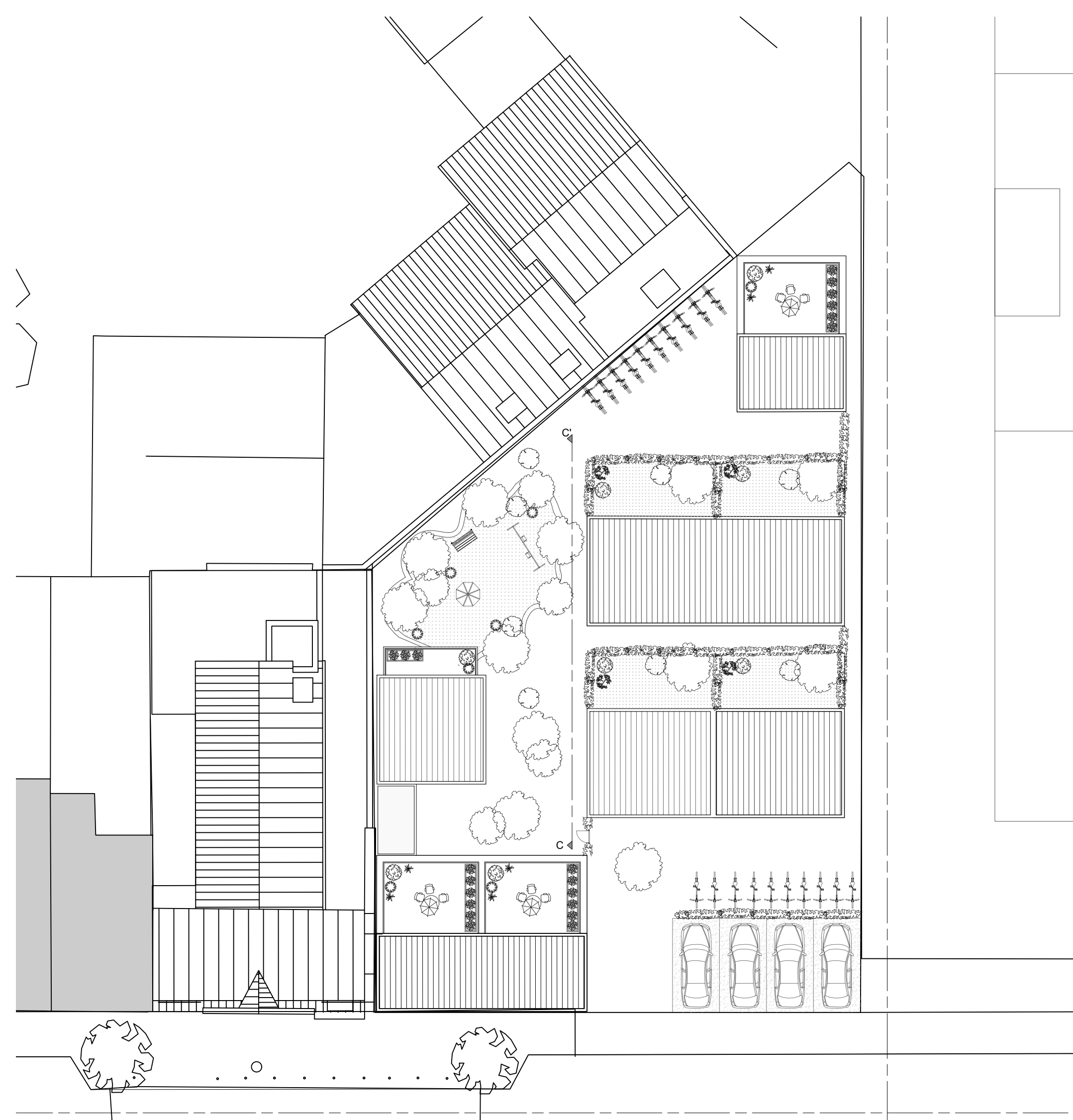
PLAN ENSEMBLE 1 / 200
